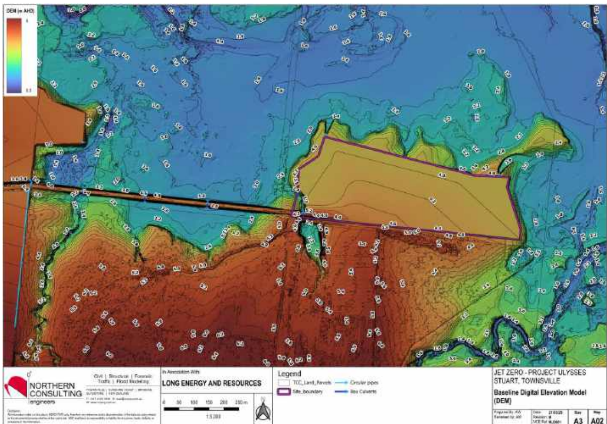
Figure 2-1 Model DEM (Inclusive of Cleveland Bay Industrial Park Far East Development)
