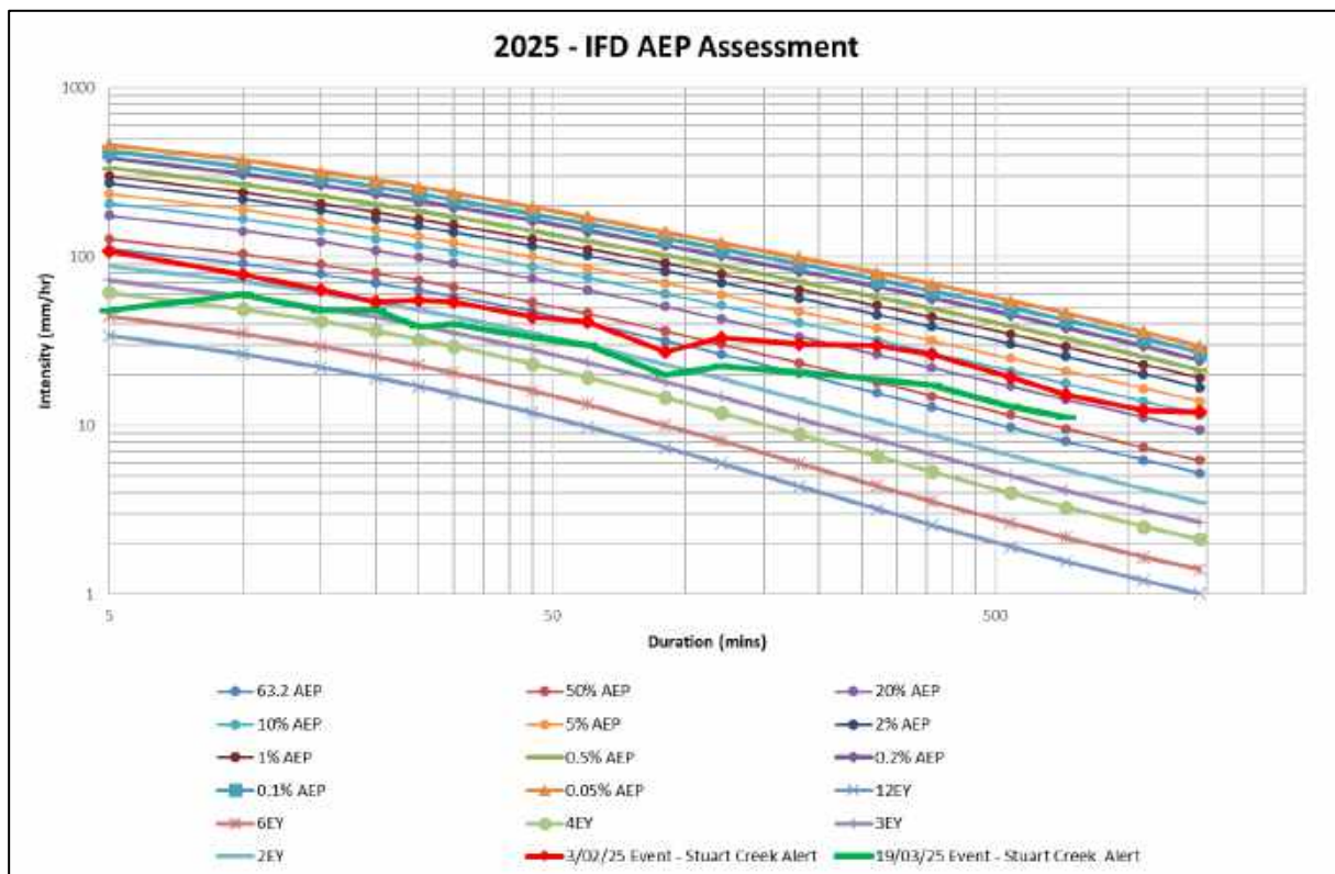
Figure 4-3 Intensity-Frequency-Duration AEP Assessment
