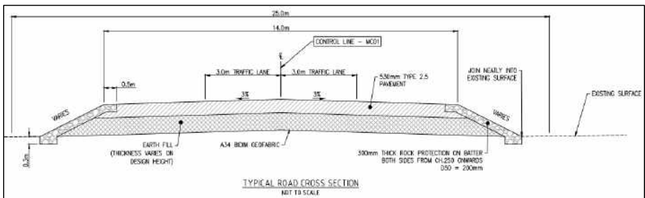
Figure 4-4 Cleveland Bay Industrial Estate - Far East Development road configuration
