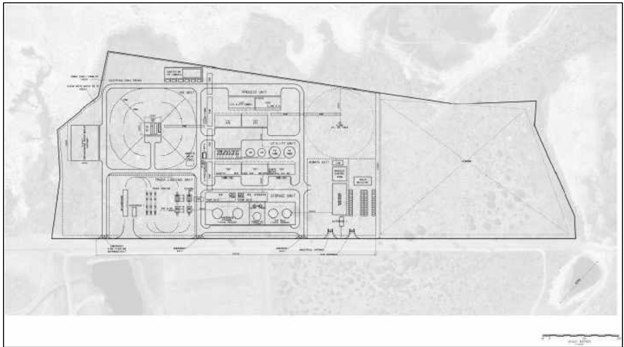
Figure 1-4 Proposed development – preliminary site layout plan
