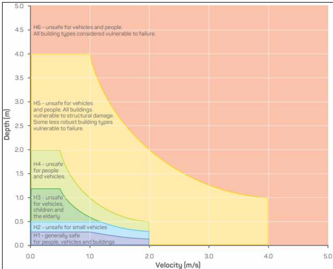
Figure 4-6 AIDR – Figure 6 - General flood hazard vulnerability curves
